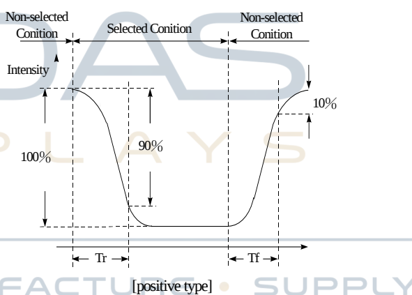
Definition of Response Time (Tr, Tf)
