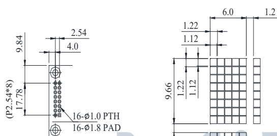
PIN DETAIL
