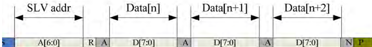
I2C master read, slave write (Slave address: 0x70)
