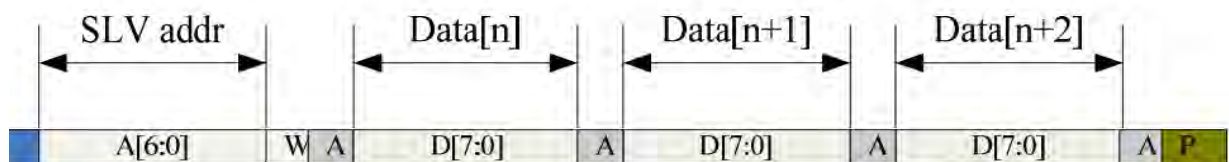
I2C master write, slave read (Slave address: 0x71)
