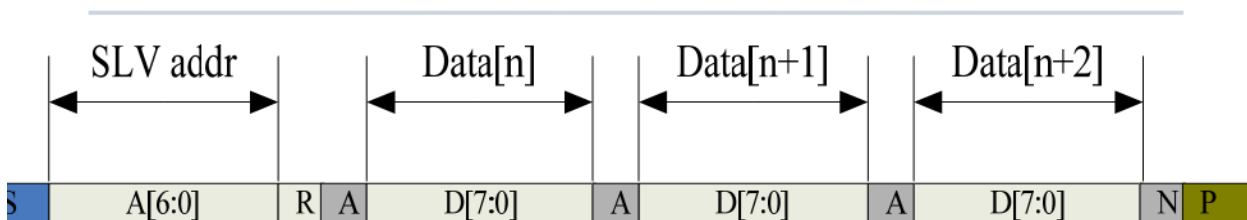
I2C master read, slave write (Slave address: 0x70)
