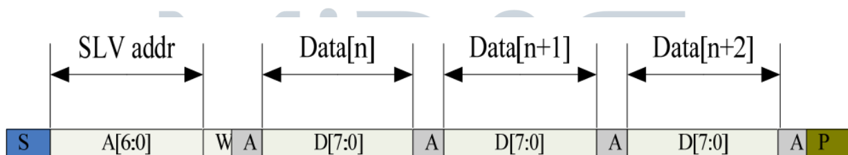
I2C master write, slave read (Slave address: 0x71)
