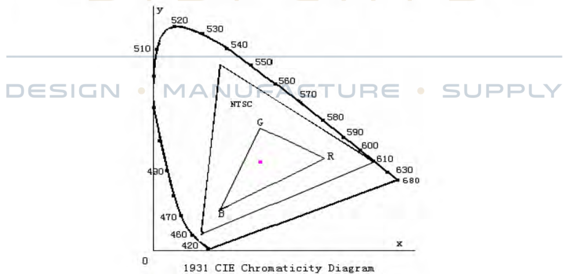
Fig. 1931 CIE chromaticity diagram
