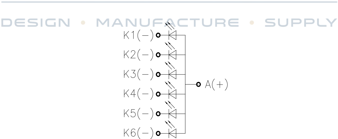
BLU CIRCUIT DIAGRAM
