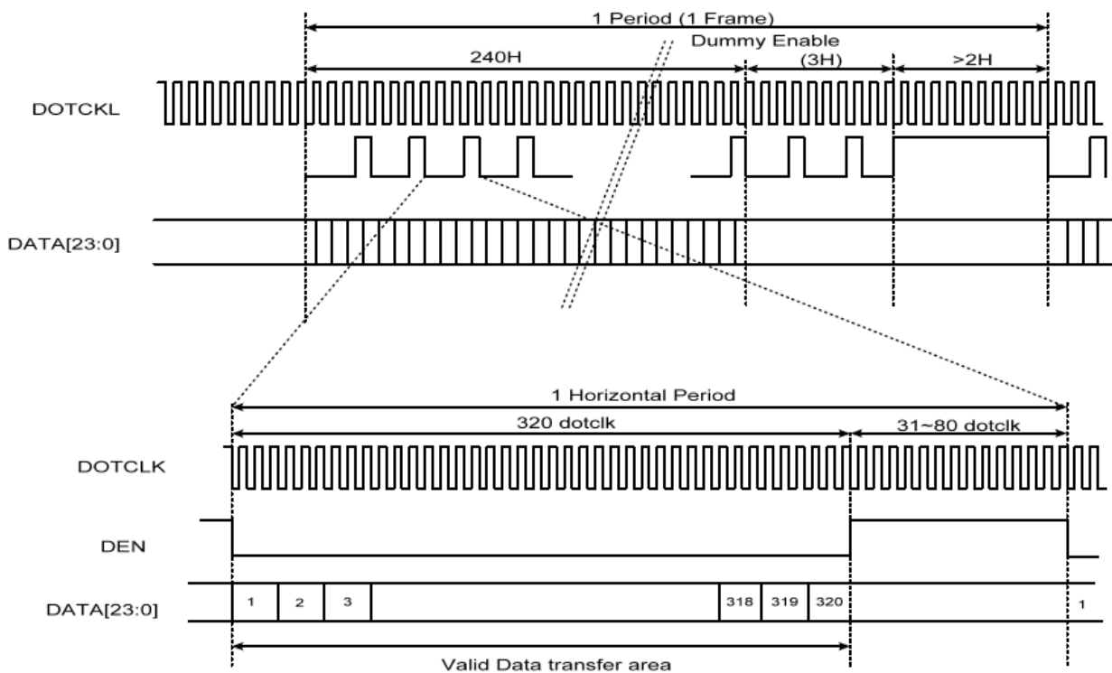
Figure 1.2 Data Transaction Timing in Parallel RGB (24 bit) Interface (IDE Mode)
