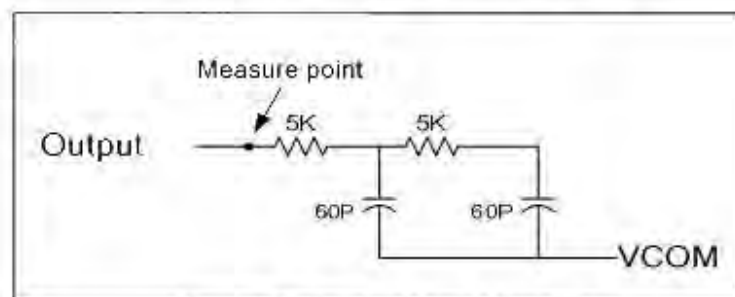
Figure 10.3 Output Load Condition
