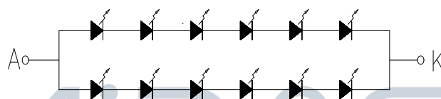
CIRCUIT DIAGRAM
