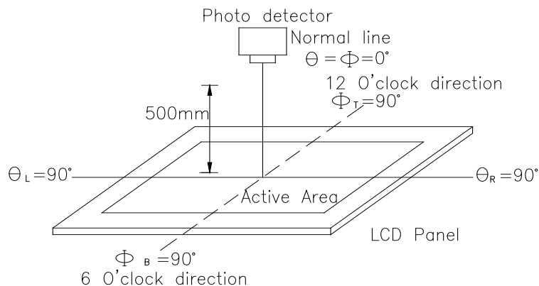
Fig. 2. Optical measurement system setup
