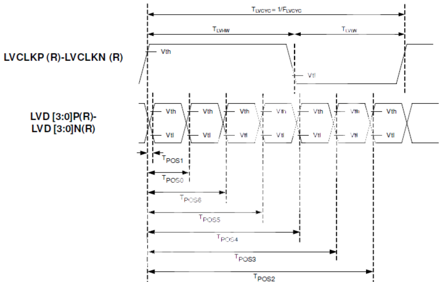
Figure 7.2: LVDS input timing
