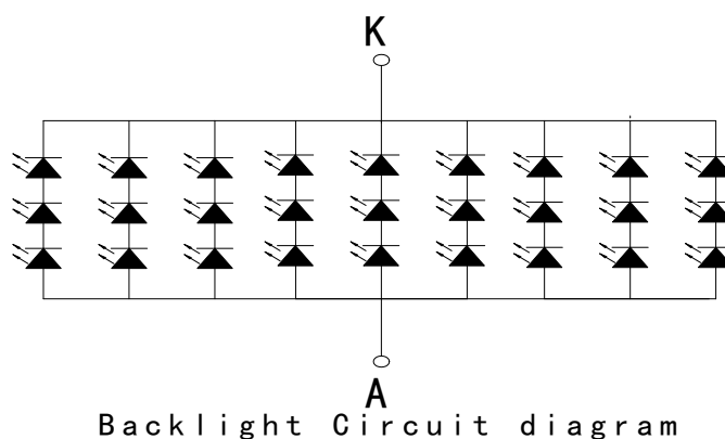
Figure : LED connection of backlight
