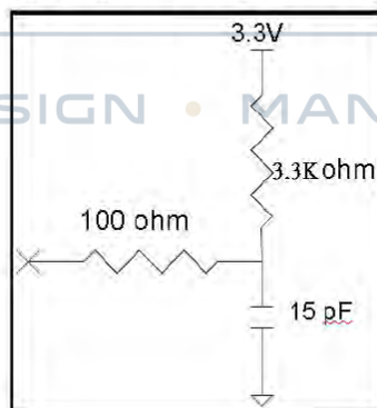
Input equivalent impedance of SDA/SCL pin
